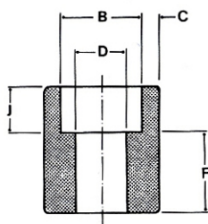
Mezzi manicotti Half couplings
