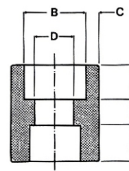
Manicotti ridotti Reducing couplings
